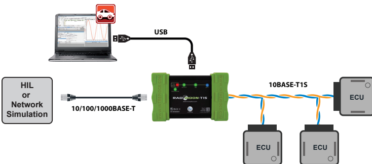
RAD-Moon T1S as a 10BASE-T1S Network Interface
