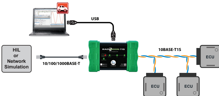
RAD-Moon T1S as a 10BASE-T1S Network Interface
