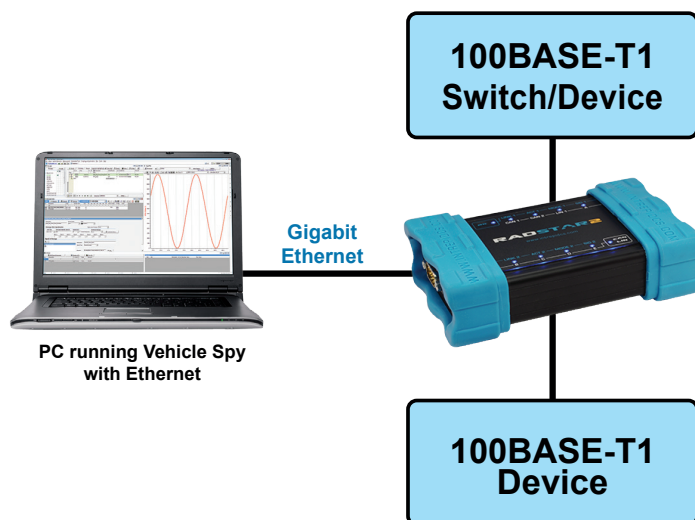
Using the RAD-Star 2 as an active tap
