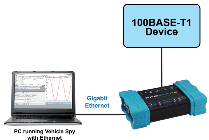
Using the RAD-Star 2 as a media converter
